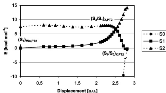
Figure 4. CAS-PT2 energy profile (energies relative to (S_1)_{Min,PT2} ) along the MEP from (S_1/S_0)_{X,PT2} to (S_1)_{Min,PT2} .
